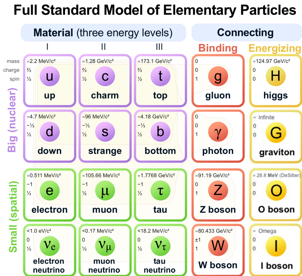
Fig. 6: Theorizing from space expansion and LENR observations one arrives at a completed or Full Standard Model of Elementary Particles with three extra energizing ones: the graviton, the out O boson and the in I boson. They operate from the fourth dimension of time and are in standard nuclear physics called scalar bosons. The big nuclear ones, in standard nuclear physics called quarks, only exist in combinations of three, thus forming the polarized proton (uud) and the neutralized neutron (ddu). Polarization with a positive proton charge and a negative electron, characterizes the first rows of the big and small material particles. (Image adapted from a Wikipedia version of the Standard Model )
