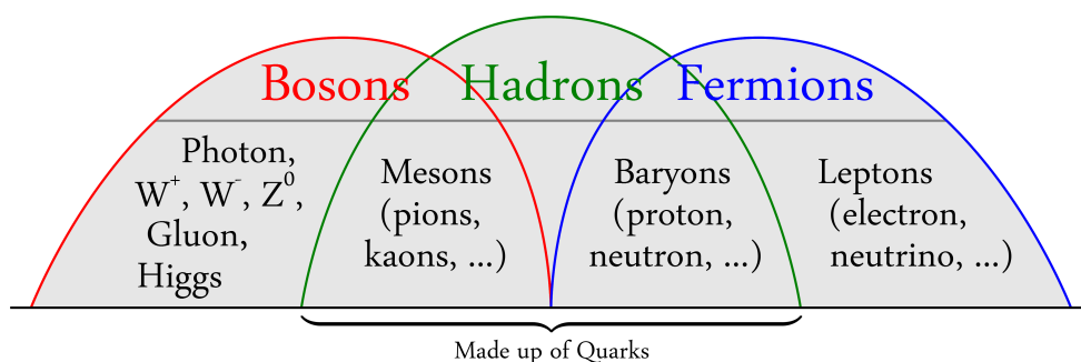
Fig. 1 The bewildering complexity of the basic categories of elementary particles of the Standard Model. The definitions overlap each other.
