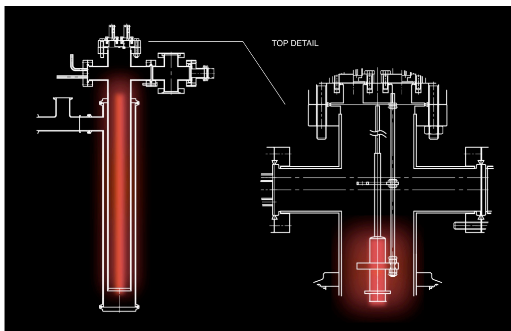
Fig. 14 A Japanese design for a LENR 2kW device prototype named Qhe Ikaros, built for industrial use, being projected for 2024. Height 63 cm, vol. 2l, weight 4kg, reactant metal:Ni & Cu, running on normal hydrogen as a (catalytic) fuel. Source: Clean Planet Co.
