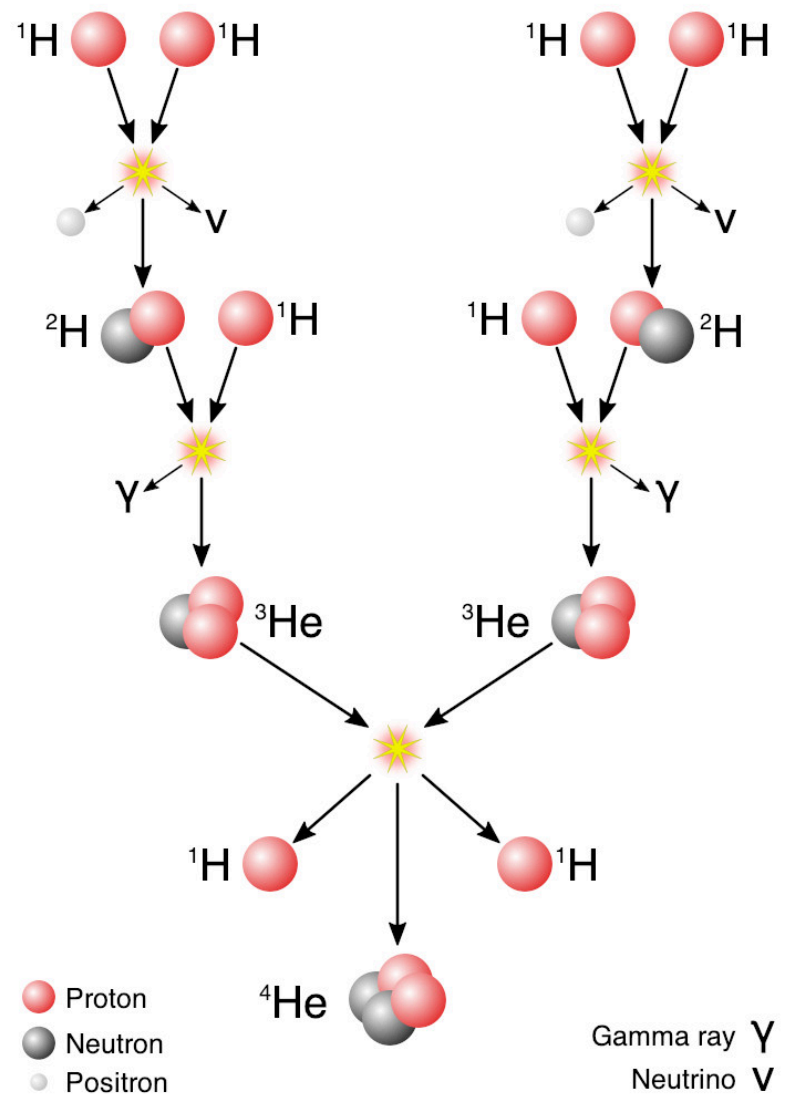
Fig 8 The by Hans Bethe defended p-p cycle of solar fusion, the supposed main source of its heat. Note the neutron appearing in the second step. Source: Wikipedia C.C.
