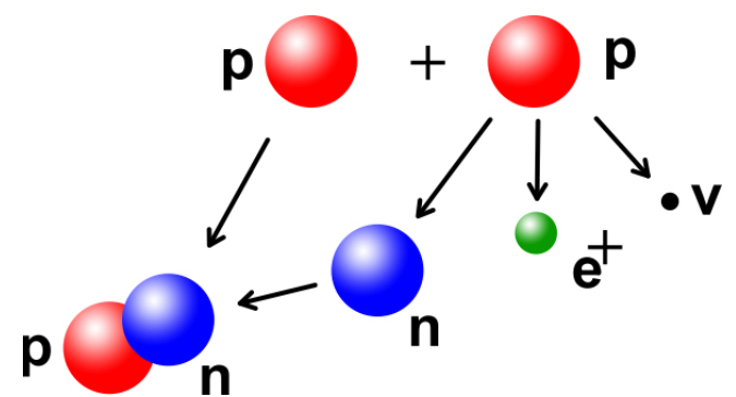
Fig 5 Protons glued together by turning one of them into a neutron first in catching an electron (not indicated) and emitting a neutrino and positron (anti-electron). Thus sticking to the proton the neutron achieves stability, in this case forming the hydrogen isotope deuterium. Source: Wikimedia C.C.
